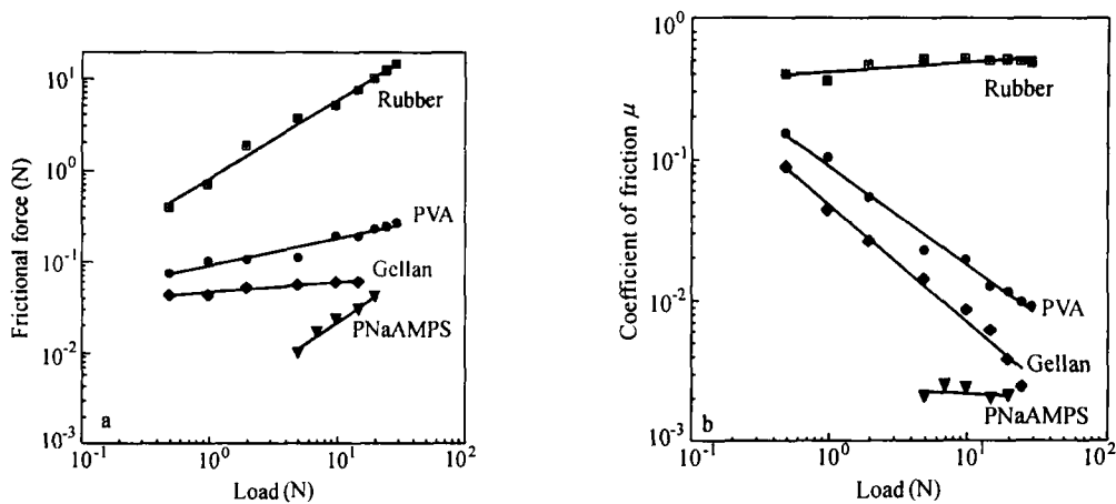
Fig. 1 Dependence of friction a) and the coefficient of friction b) on load for various kinds of hydrogels sliding on a glass surface in air Sliding velocity: 7 mm/min; sample contact area: PVA, gellan and rubber, 3 × 3 cm 2 , PNaAMPS, 2 × 2 cm 2 ; degree of swelling q : PVA, 17; gellan, 33; PNaAMPS, 15
