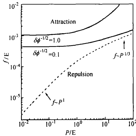
Fig. 3 Pressure dependence of the frictional forces for gels sliding on a repulsive substrate (dotted line) as well as on attractive substrates with various \delta\phi^{1/2} (solid lines)
