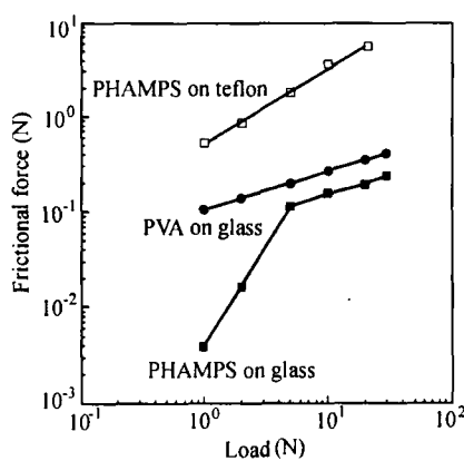
Fig. 2 Load dependence of gel friction in water Sliding velocity: 90 mm/min; gel size: PVA, 3 × 3 × 0.8 cm 3 ; PHAMPS, 3 × 3 × 0.6 cm 3 ; degree of swelling: PVA, q = 10 ; PHAMPS, q = 15
